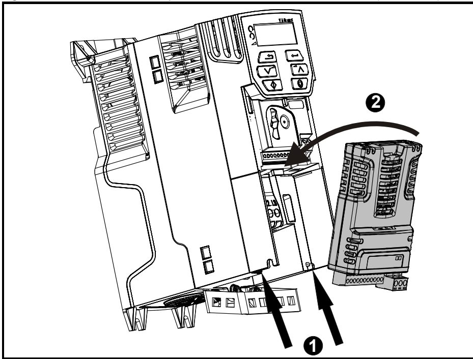
Figure 3-1 Installation of an SI option module on Unidrive M200 to M400 (sizes 2 to 4)
