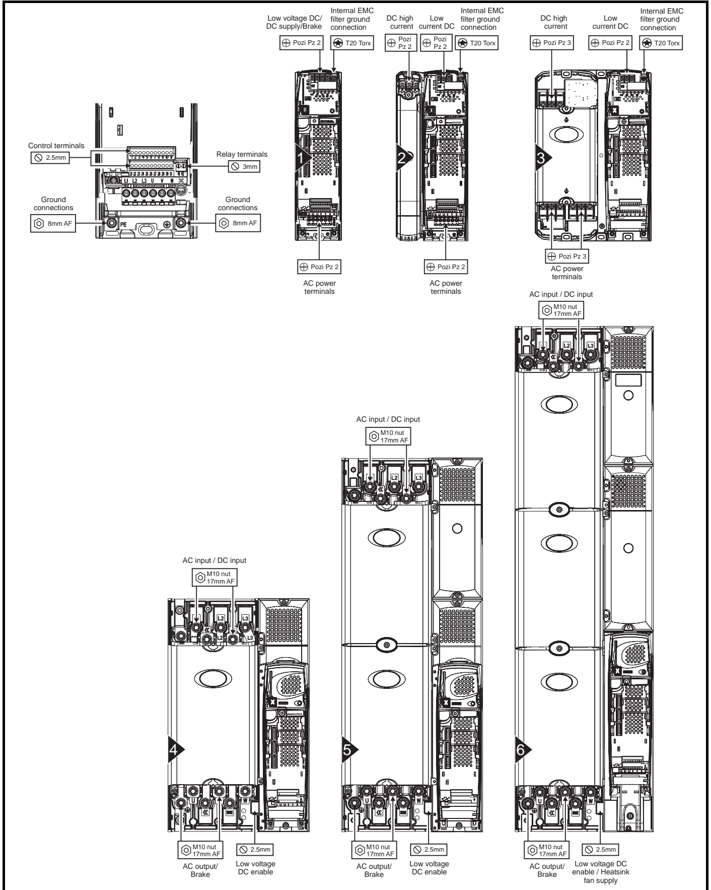
Figure 3-65 Locations of the power and ground terminals on wall mounted drives
