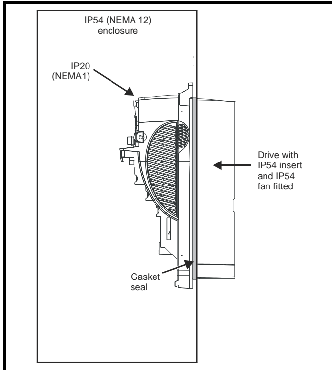
Figure 3-44 Example of IP54 (NEMA 12) rating layout
