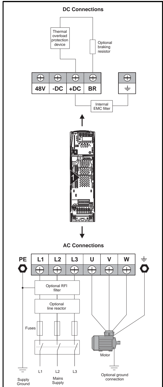
Figure 4-1 Unidrive SP size 1 power connections
