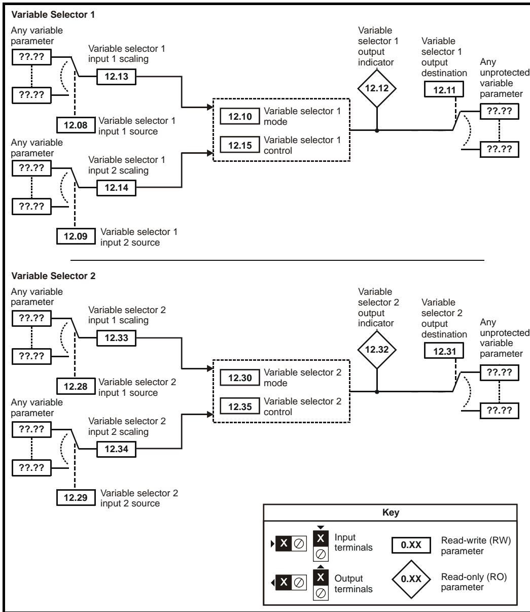
Figure 11-15 Menu 12 logic diagram (continued)
