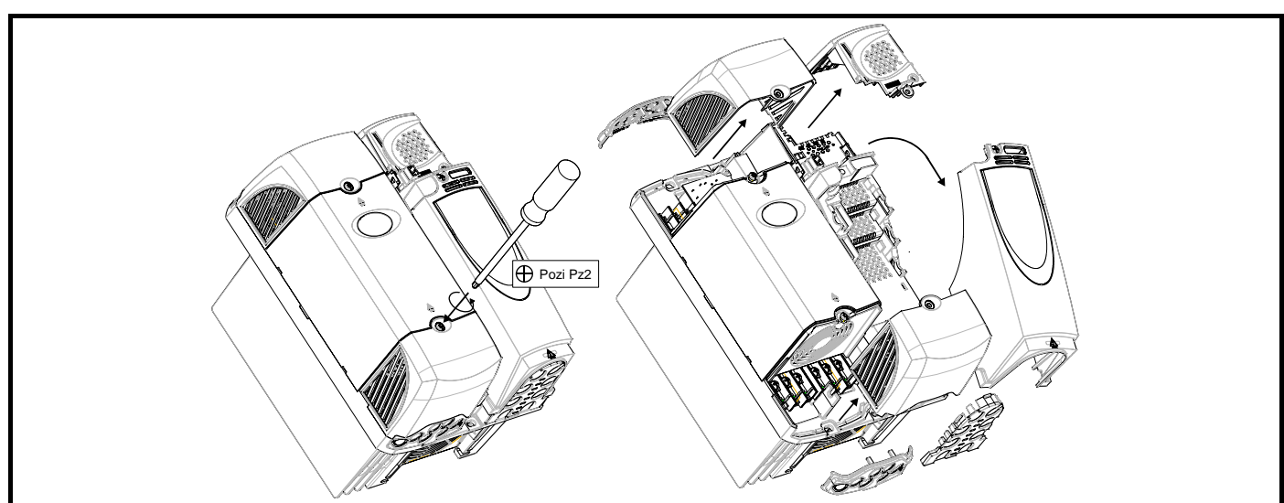
Figure 3-7 Removing the size 3 terminal covers
