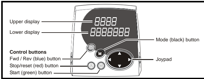
Figure 5-1 SM-Keypad
