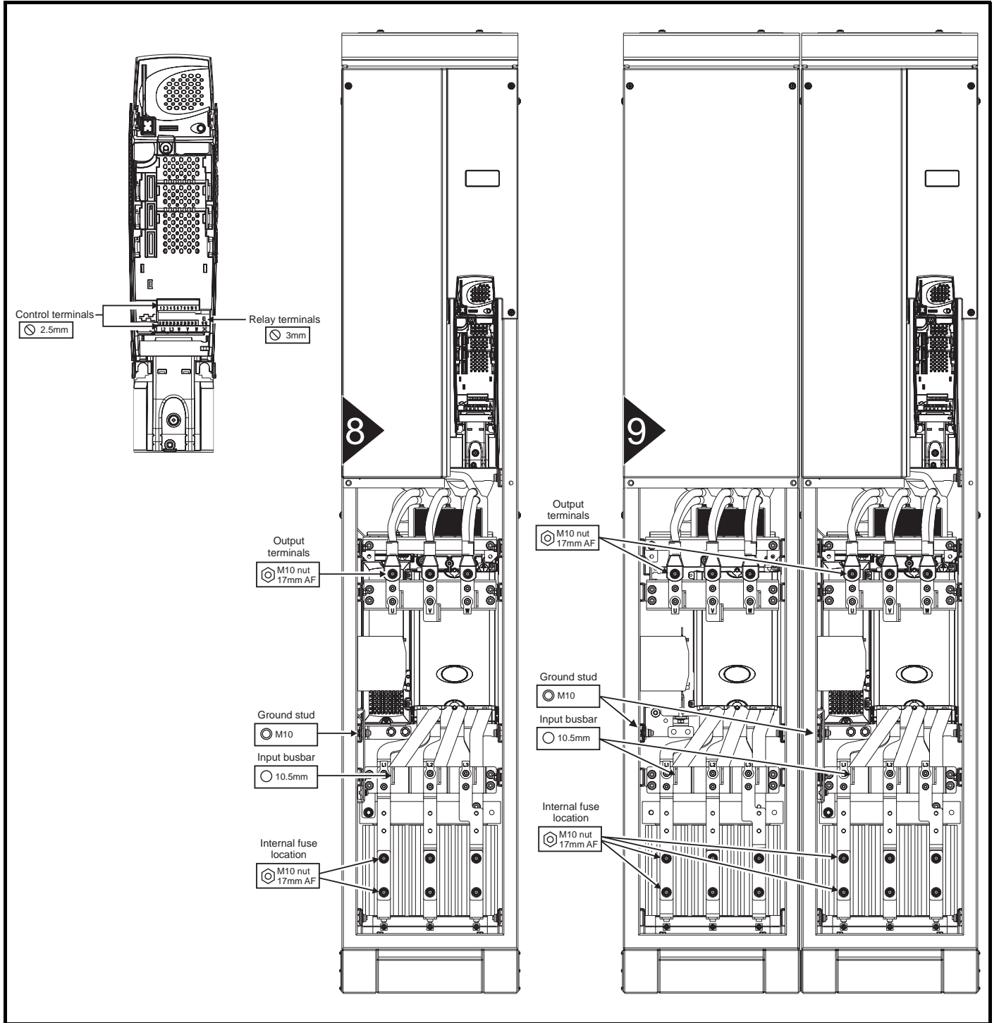
Figure 3-66 Locations of the power and ground terminals on free standing cubicle drives
