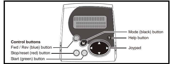
Figure 5-2 SM-Keypad Plus
