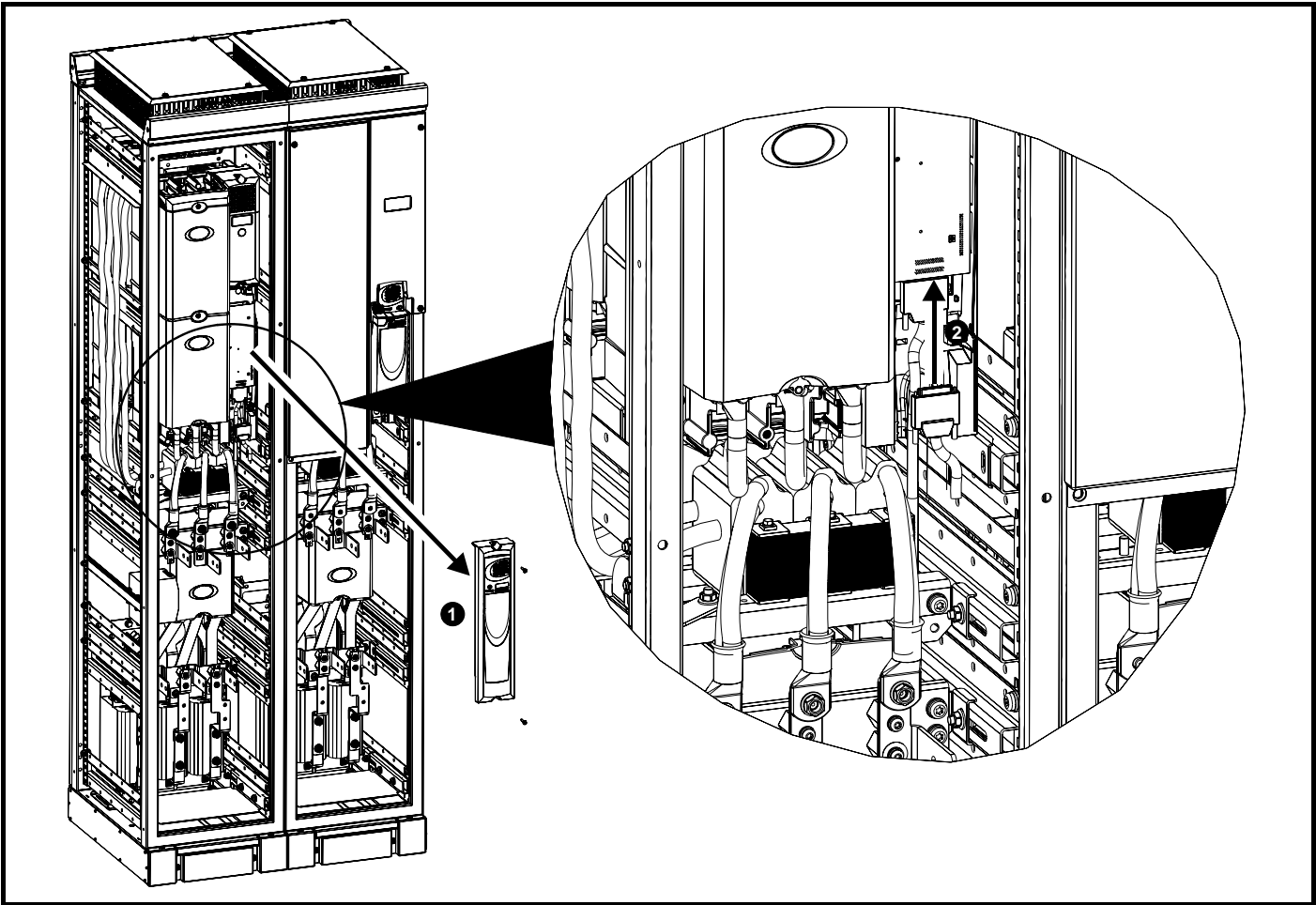
Figure 3-17 Fitting the parallel cable from a size 9 master to slave
