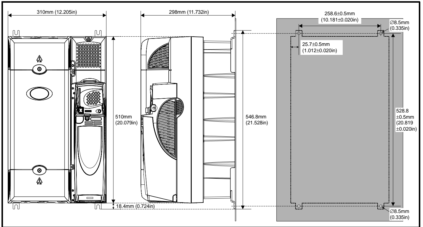
Figure 3-27 Surface mounting the size 4 drive
