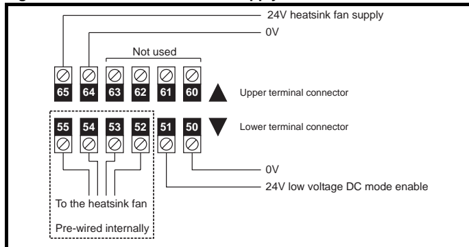
Figure 4-12 Size 6 heatsink fan supply connections
