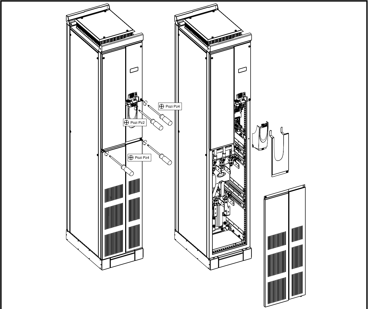
Figure 3-9 Removing the size 8 terminal covers from the free standing cubicle drive
